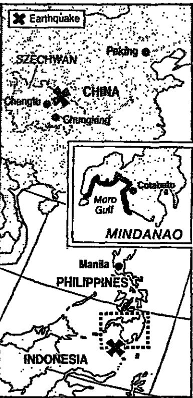
Where the earthquakes were centered (marked by X's) in China and the Philippines, and the coastline of Mindanao where the tidal waves struck (inset).
